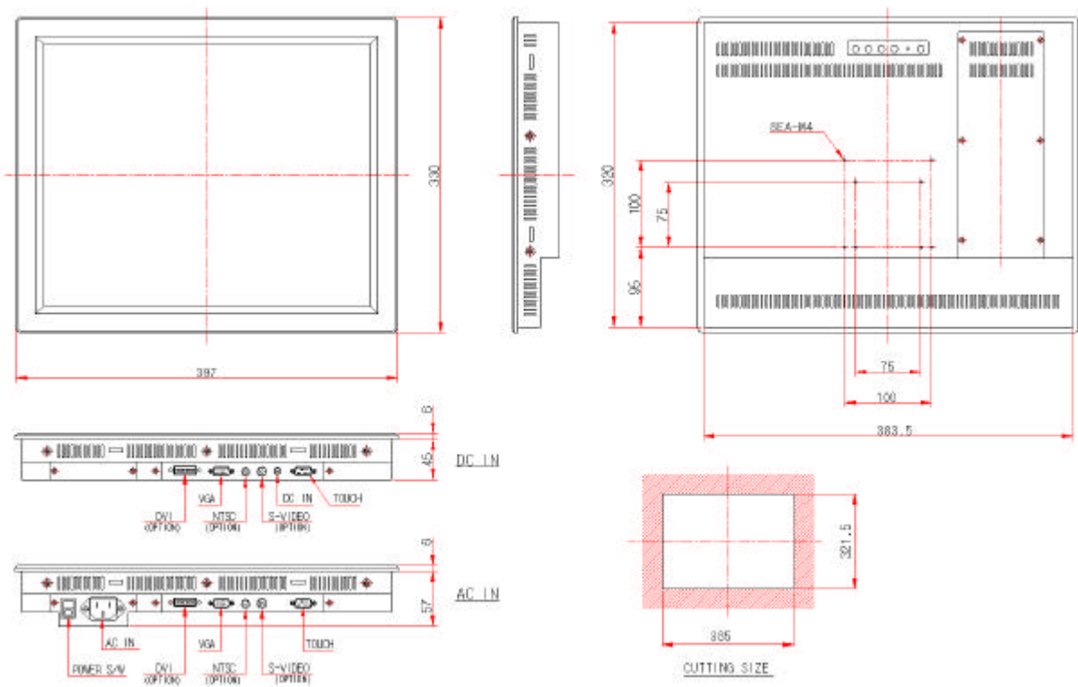
Monitor Dimensions
